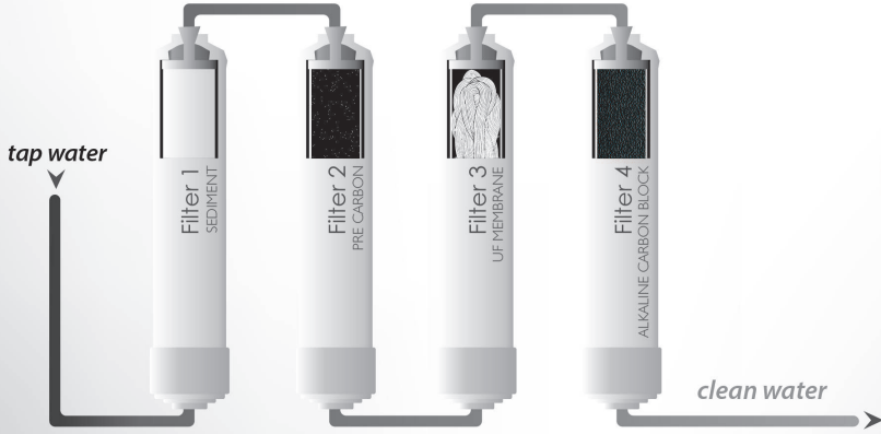
Filter - 1 SEDIMENT
